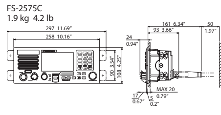
Control unit FS-2575C
